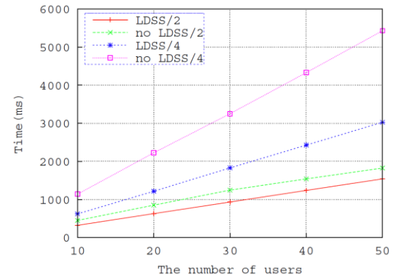
Fig. 10. The overhead of attribute revocation.
