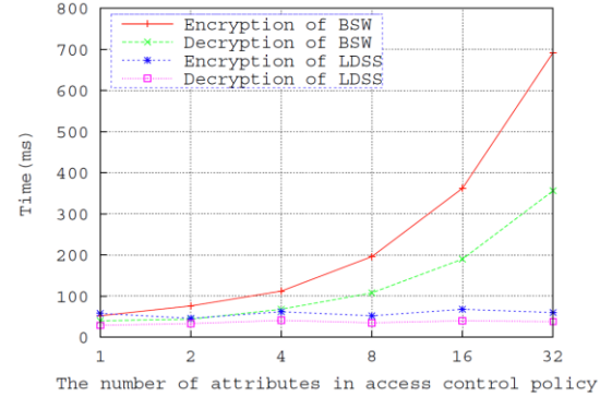
Fig. 9. The relationship between users' overhead and the size of access control policy.
