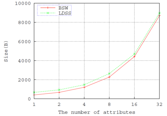
Fig. 12. The storage overhead of SK.
